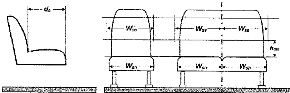
Figure 5. Seat dimensions
