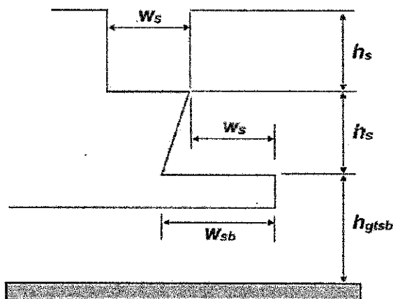
Figure 7. Step board
