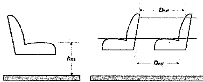
Figure 6. Seat layout
