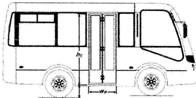
Figure 8. Service door dimensions
