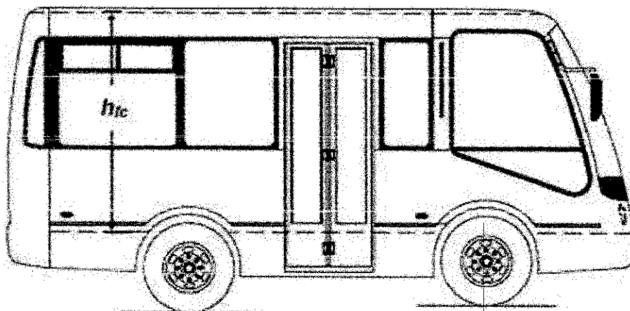
Figure 3. Floor-to-ceiling height
